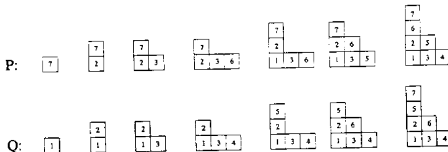
FIG. 4 - Algorithme de Robinson-Schensted
